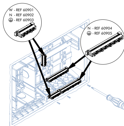
INSTALLATION OF BRASS TERMINALS
